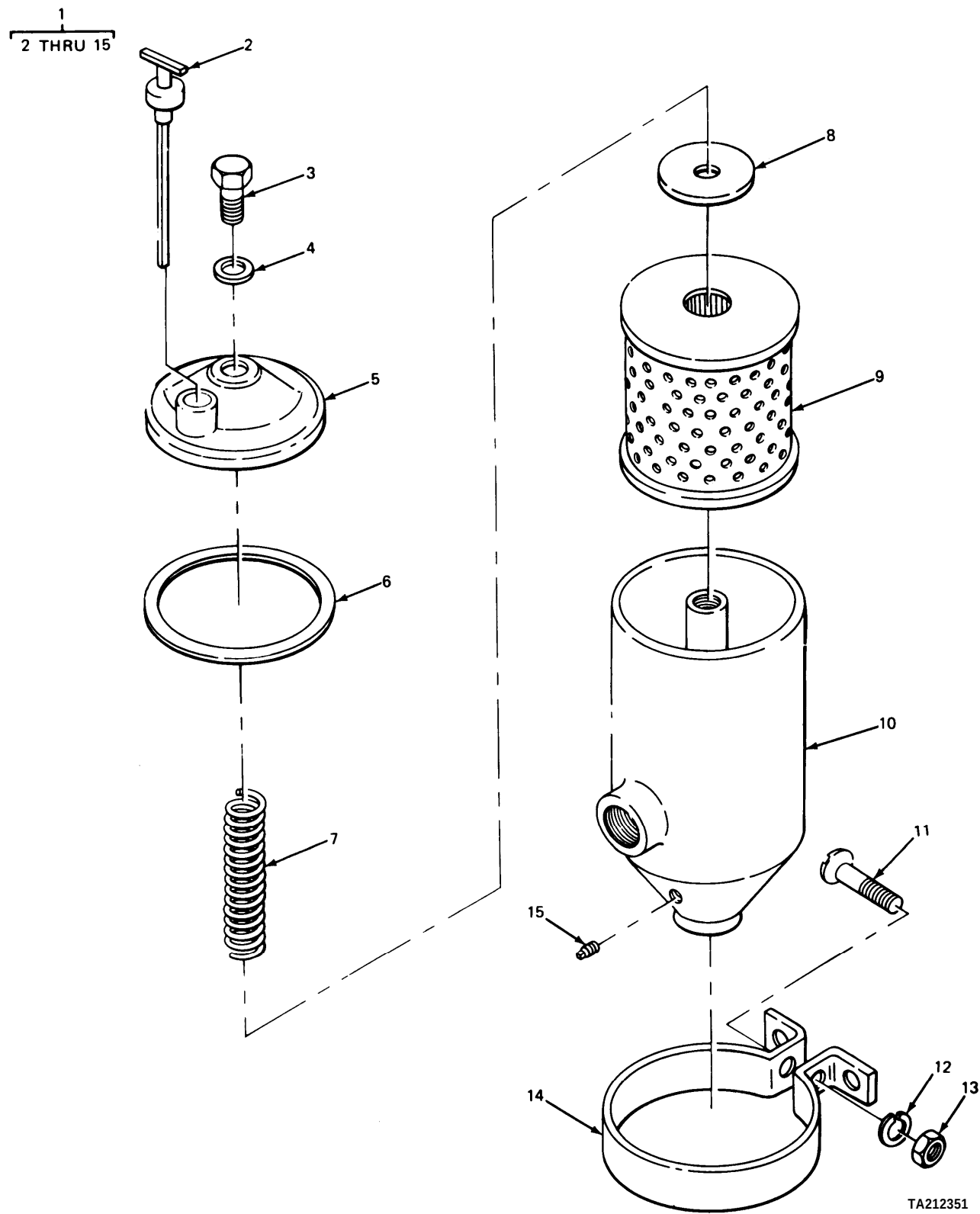
FIGURE 226. RESERVOIR AND FILTER ASSEMBLY.
