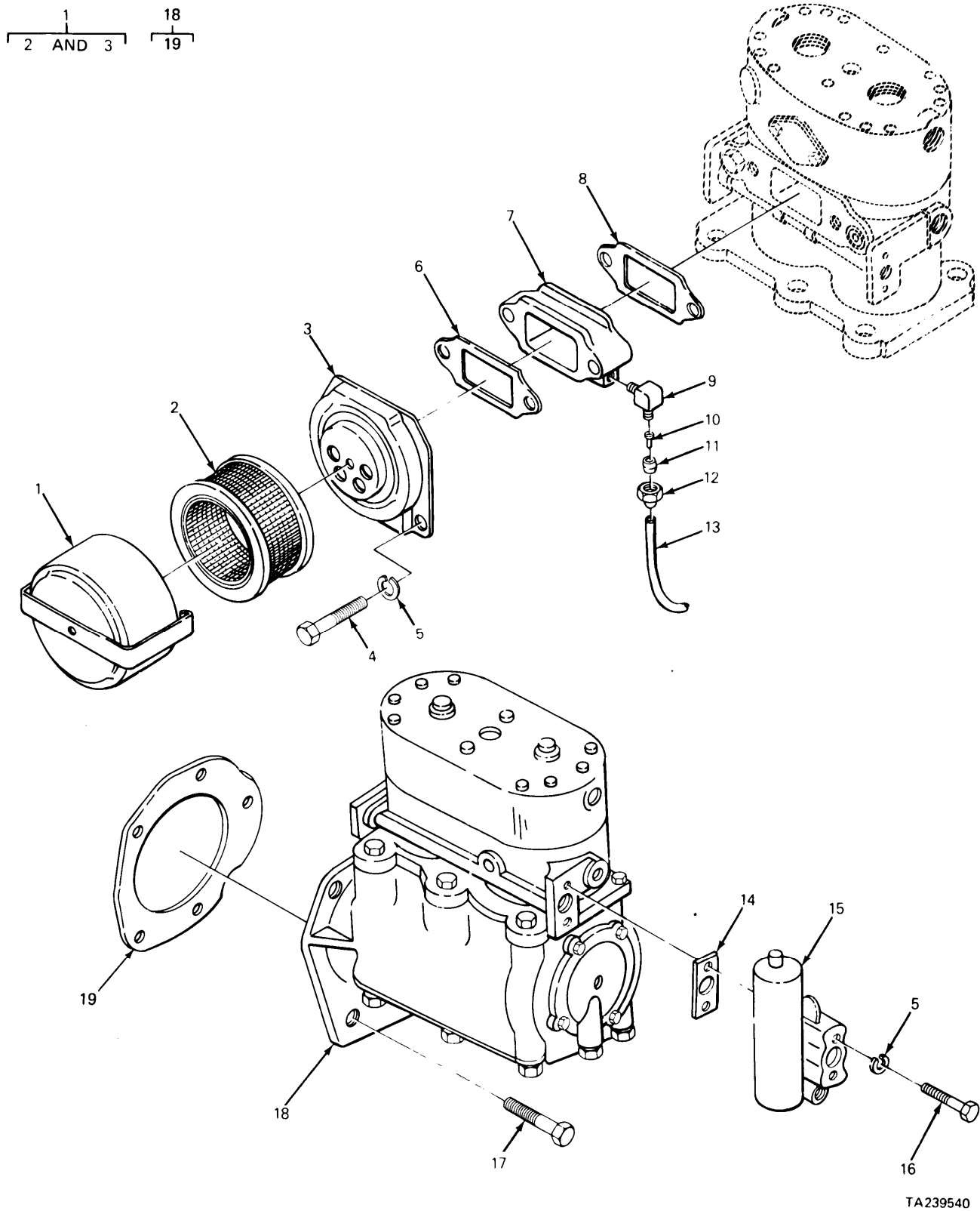
FIGURE 197. AIR COMPRESSOR AND RELATED PARTS.
