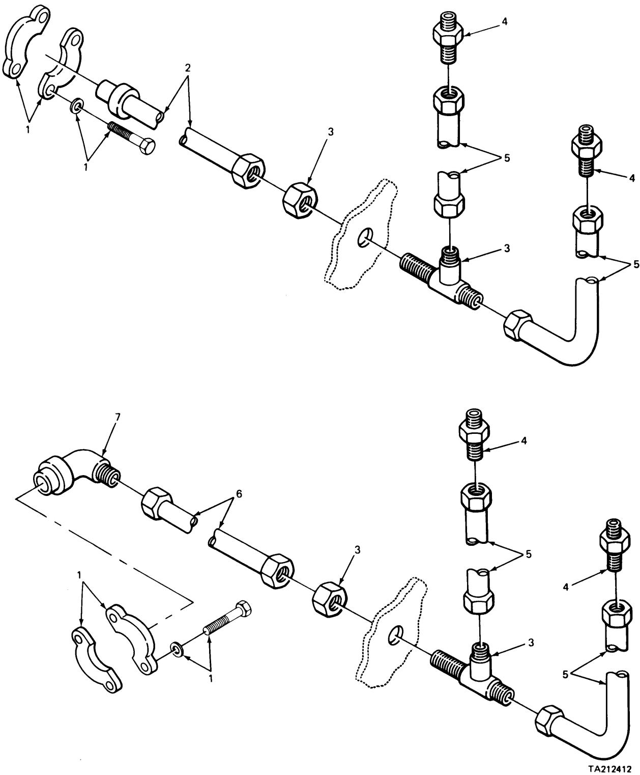
FIGURE 287. ADAPTERS FOR HYDRAULIC WINCH.
