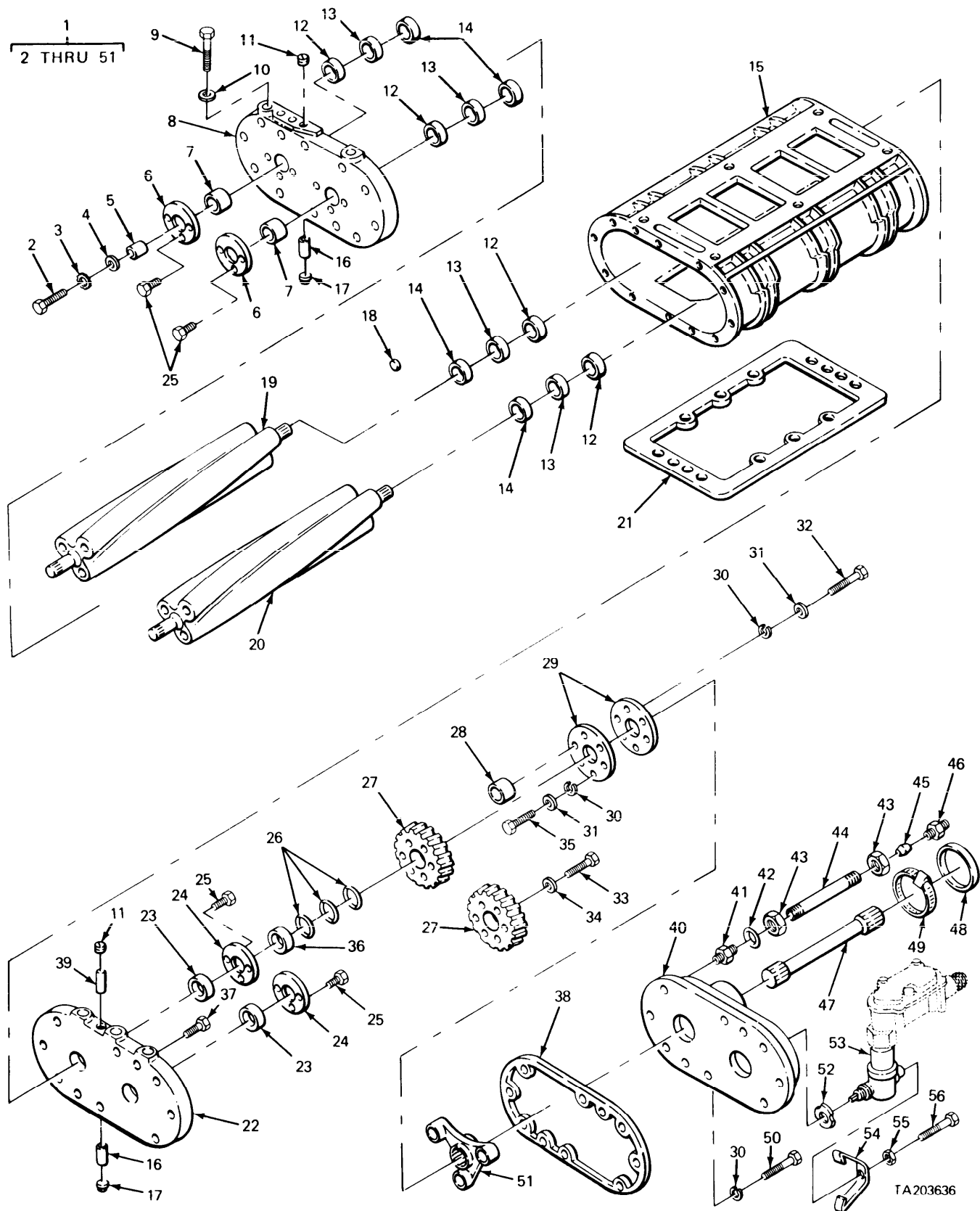
FIGURE 43. BLOWER EXPLODED VIEW.
