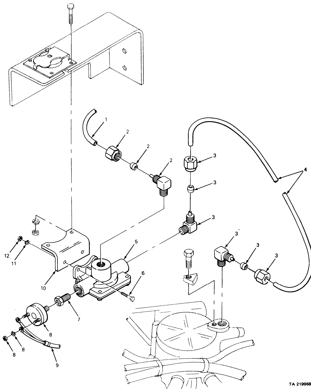
FIGURE 208. QUICK RELEASE VALVE AND ATTACHING PARTS.
