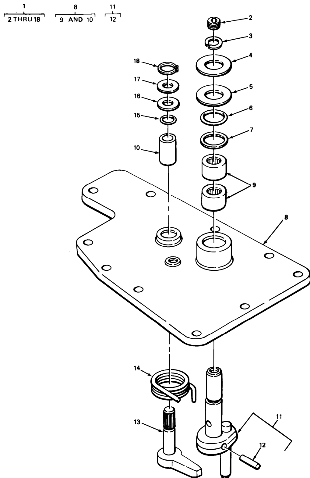
FIGURE 49. GOVERNOR COVER AND RELATED PARTS.
