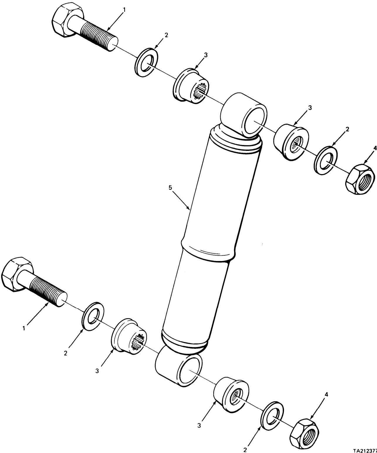
FIGURE 249. SHOCK ABSORBER.
