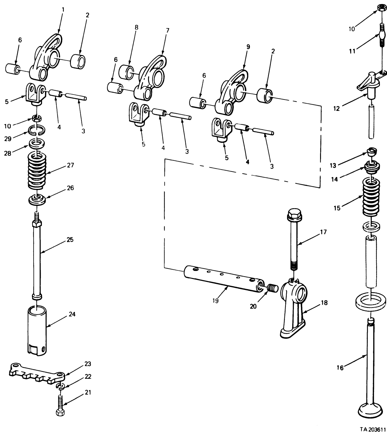
FIGURE 15. VALVES, TAPPETS, ROCKER ARMS, AND RELATED PARTS.
