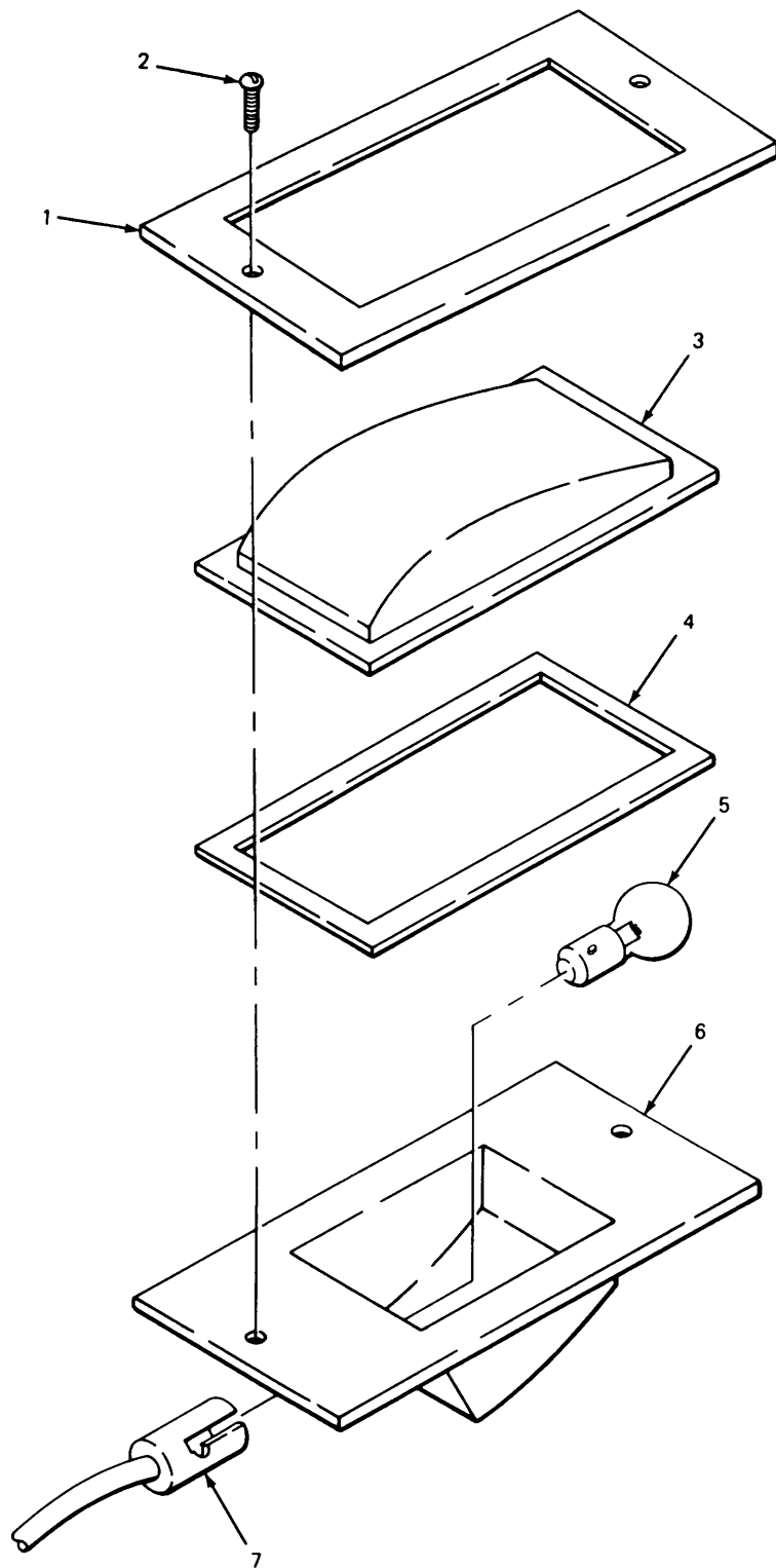
FIGURE 82. DOME LIGHT.
