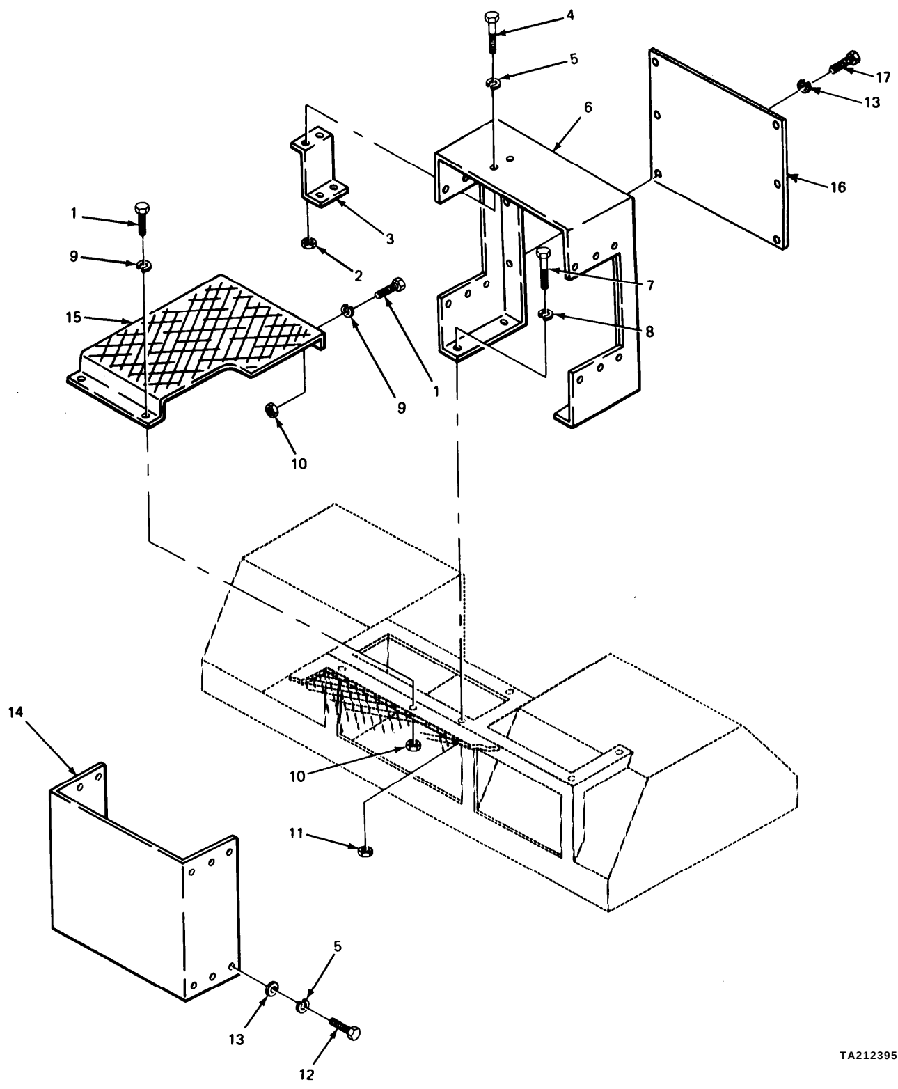
FIGURE 269. CONSOLE PANEL AND RELATED PARTS.
