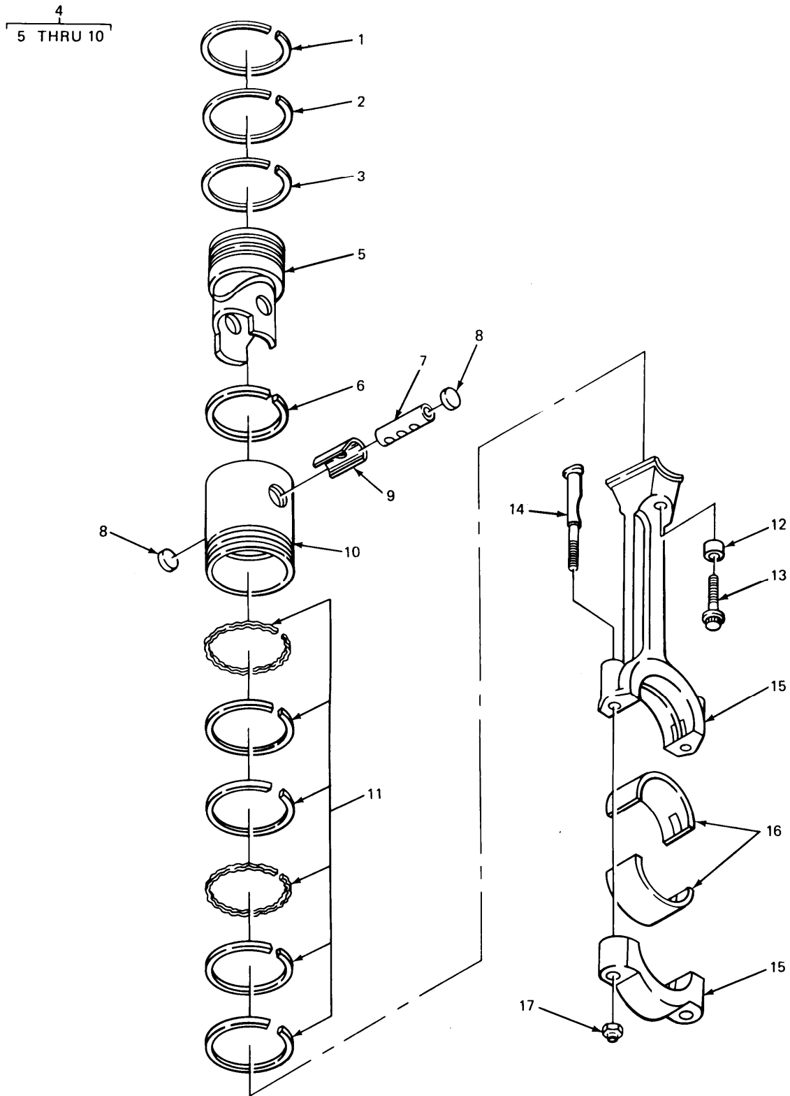
FIGURE 13. PISTON, RINGS, CONNECTING ROD AND RELATED PARTS.
