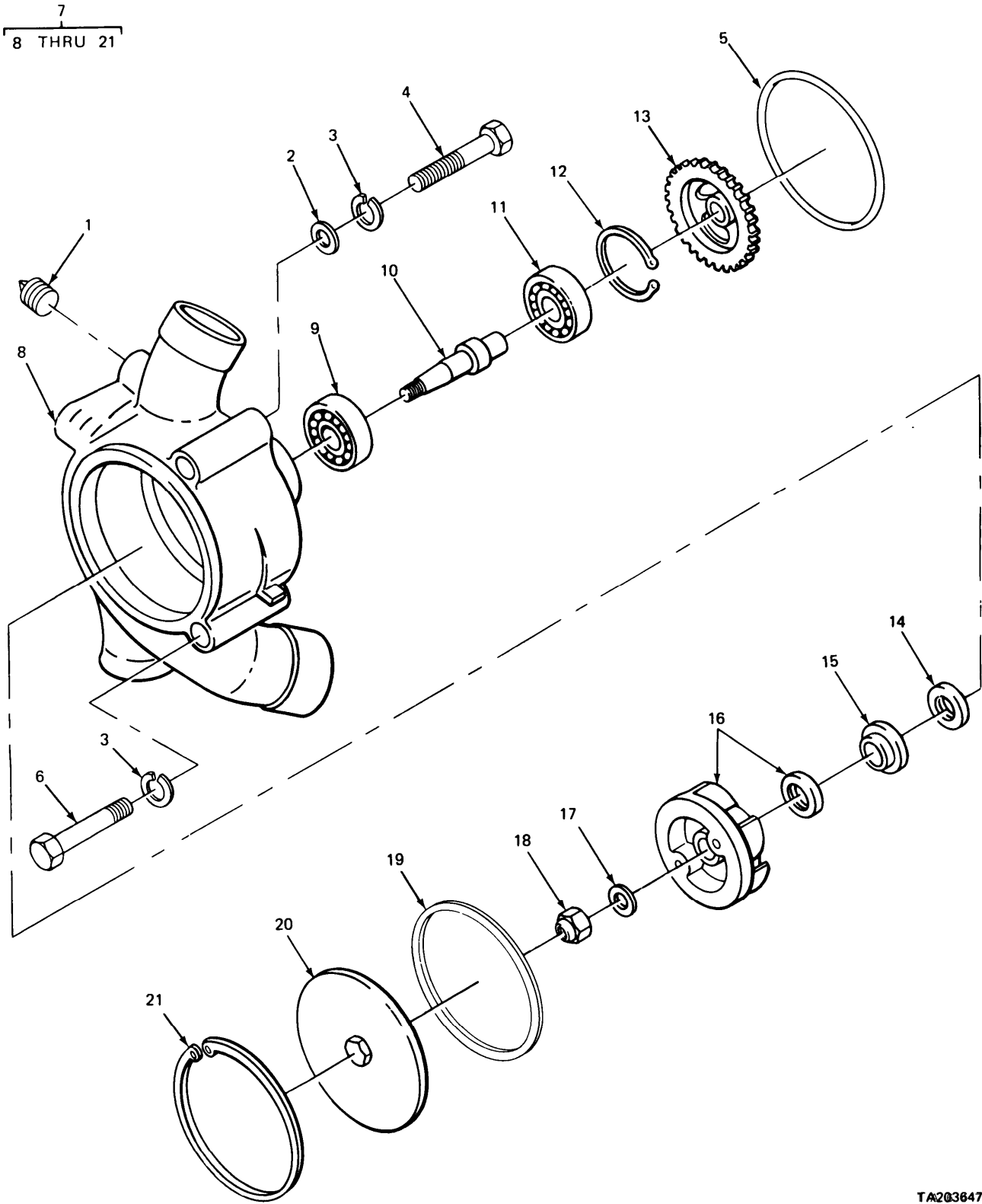
FIGURE 67. WATER PUMP.
