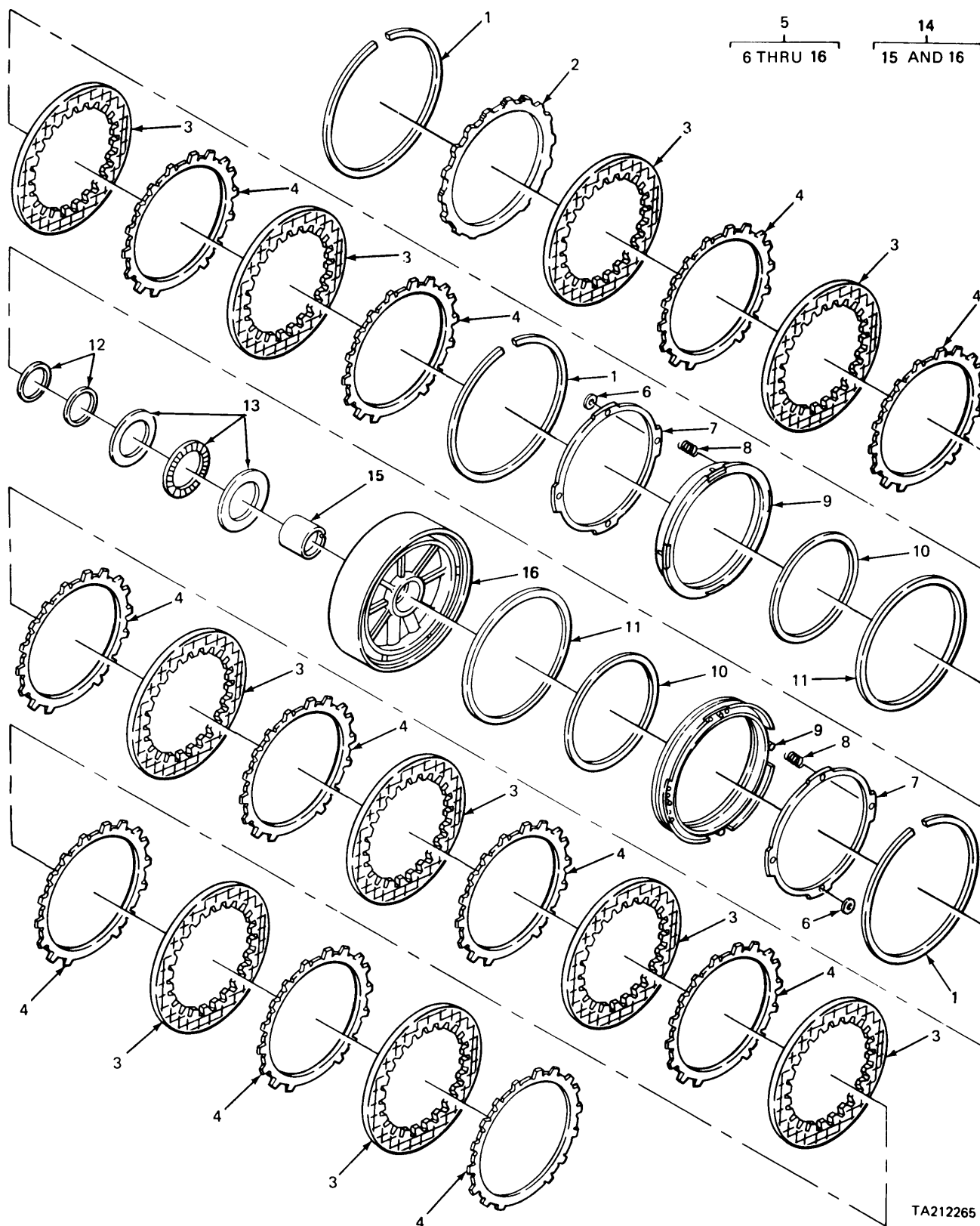
FIGURE 123. CLUTCH SUPPORT ASSEMBLY FOR CENTER, THIRD AND FOURTH CLUTCH.
