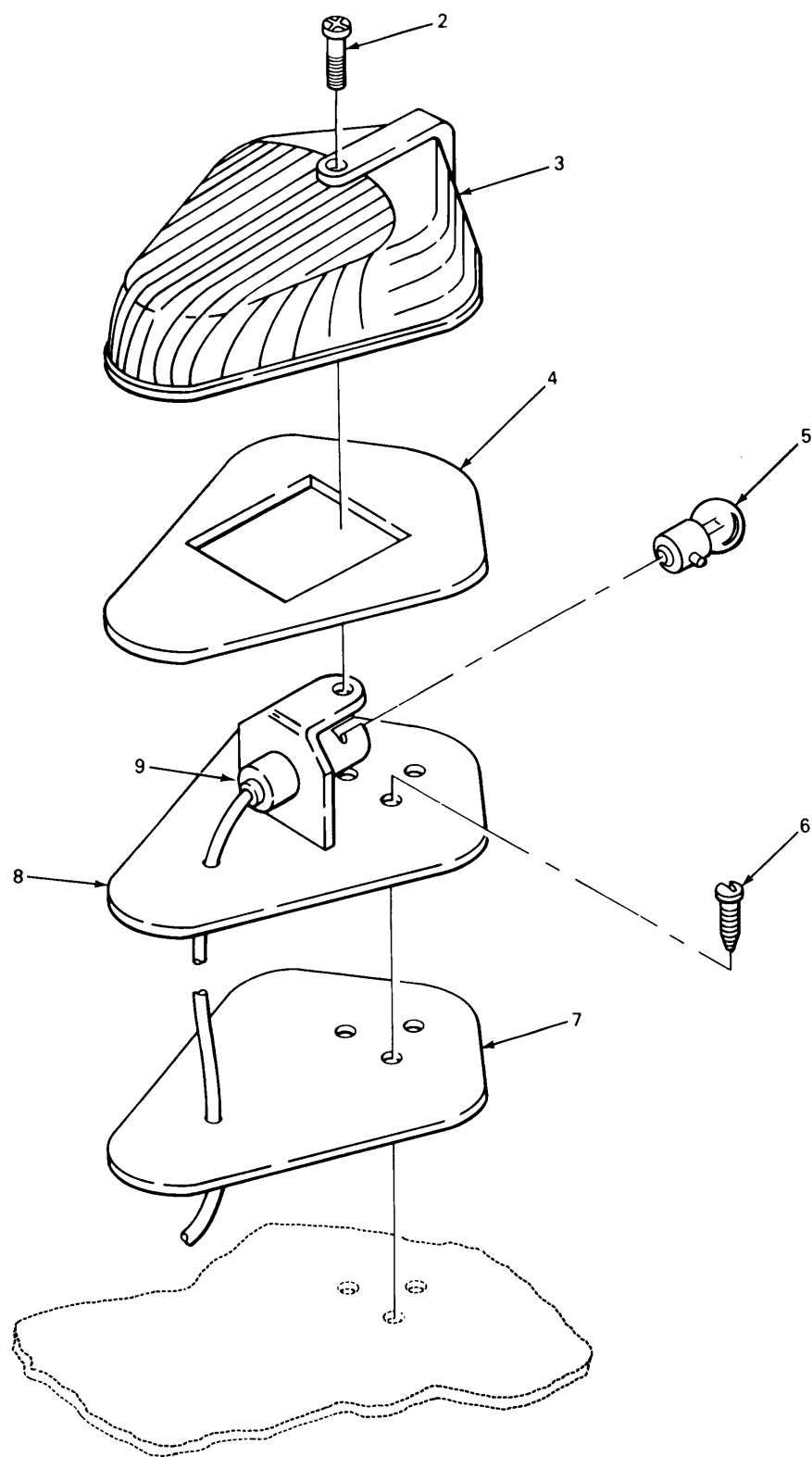
FIGURE 84. CLEARANCE LIGHT.
