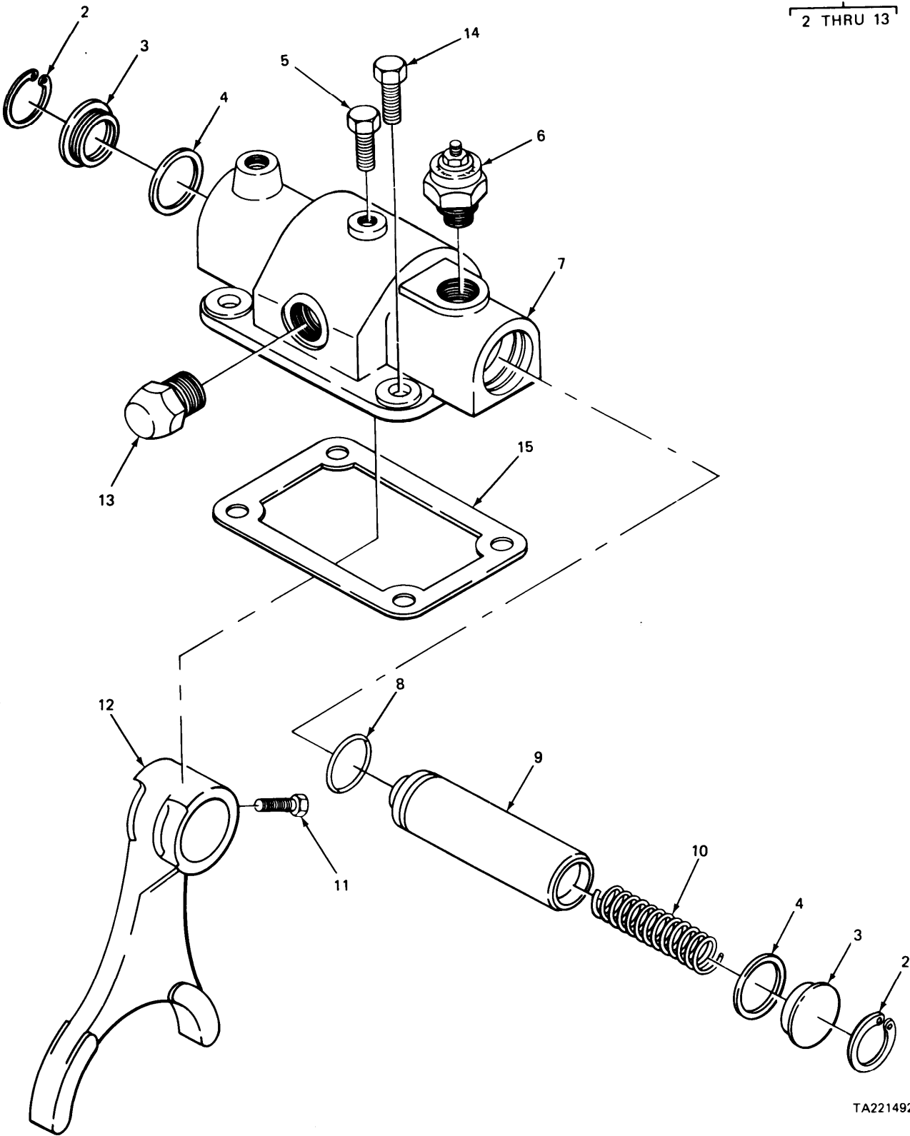
FIGURE 285. AIR SHIFT ASSEMBLY, P. T. O..
