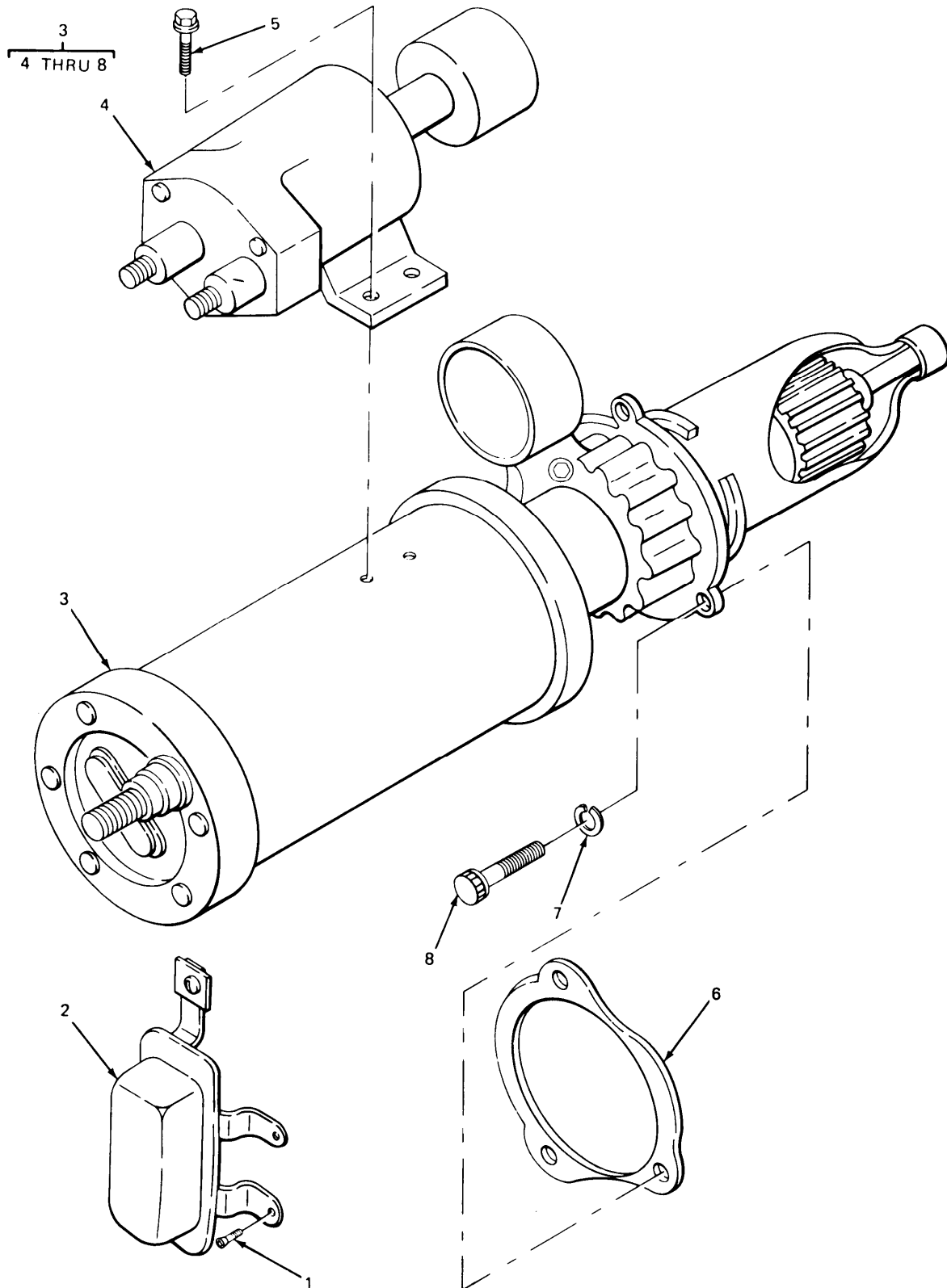
FIGURE 72. STARTER, RELAY, SOLENOID AND RELATED PARTS.
