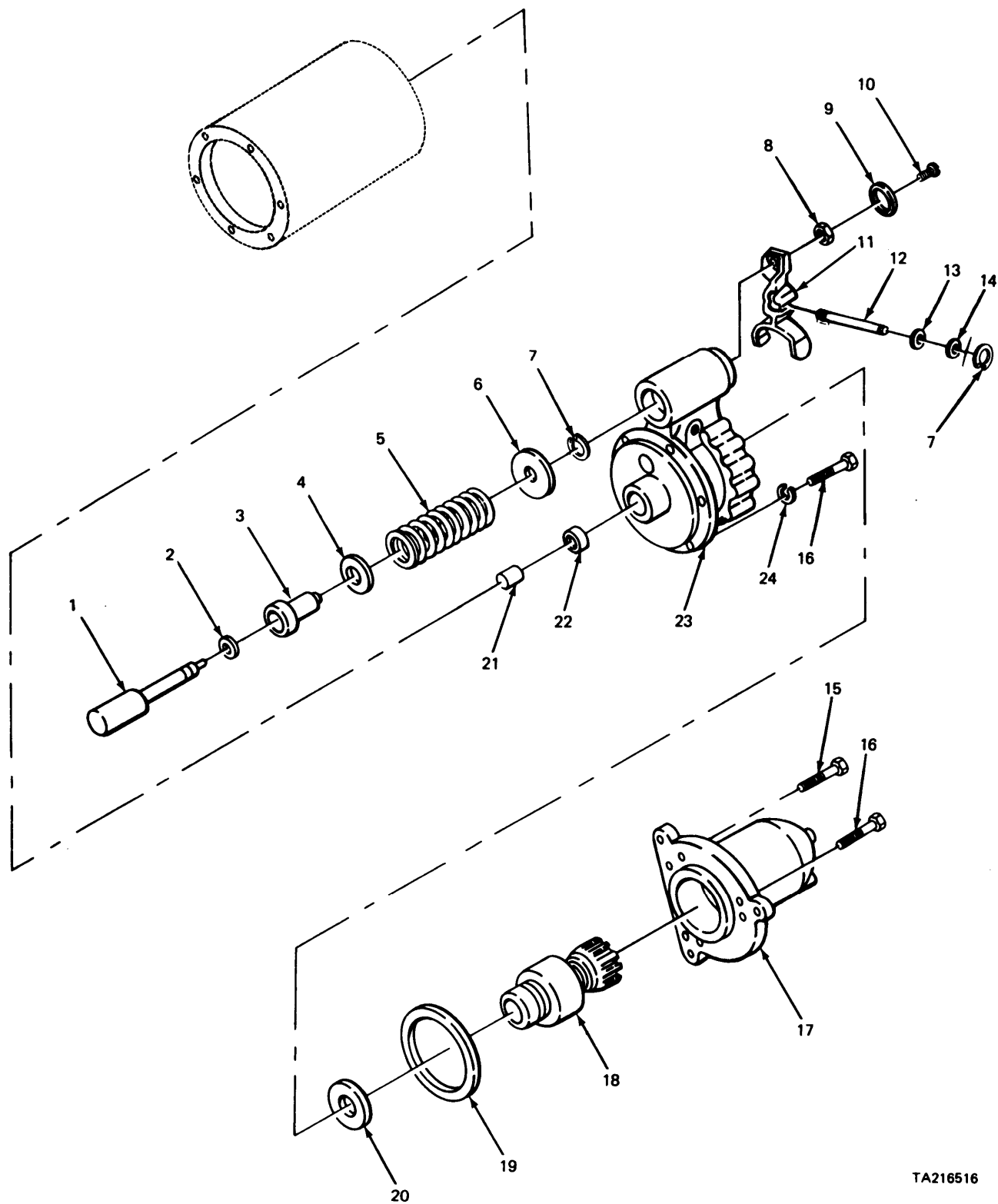
FIGURE 74. STARTER LEVER HOUSING AND RELATED PARTS,
