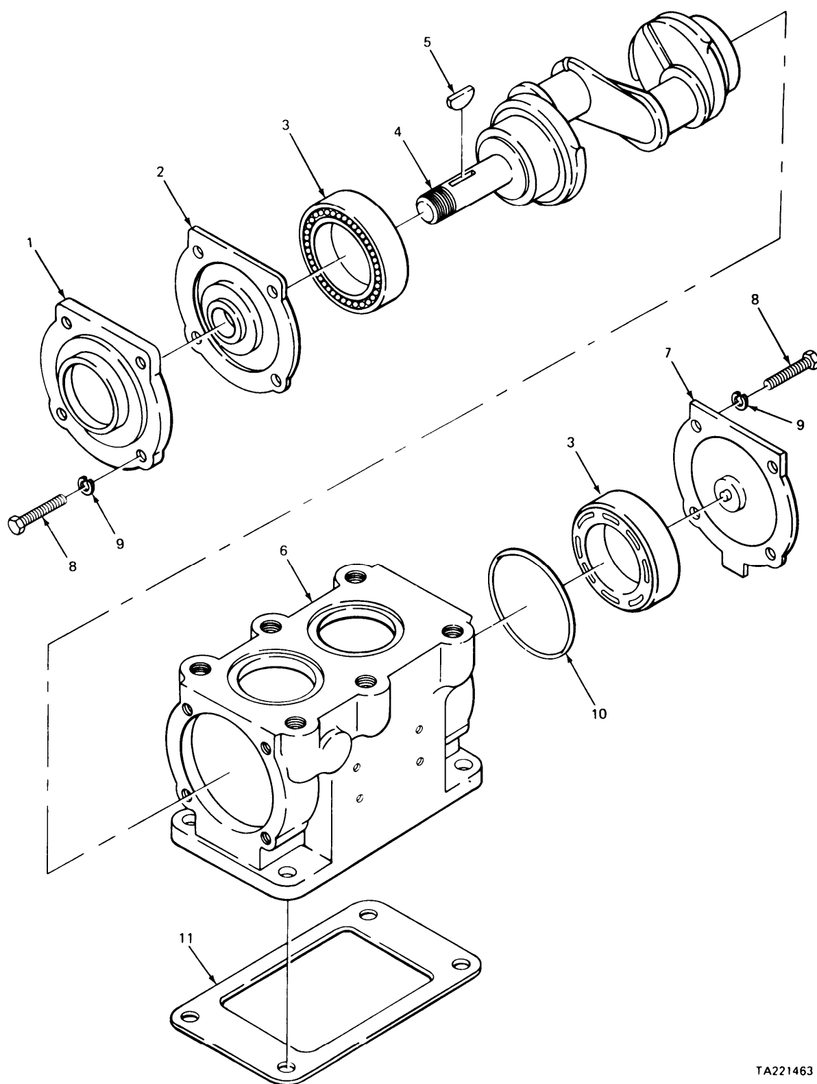
FIGURE 199. AIR COMPRESSOR CRANKCASE.
