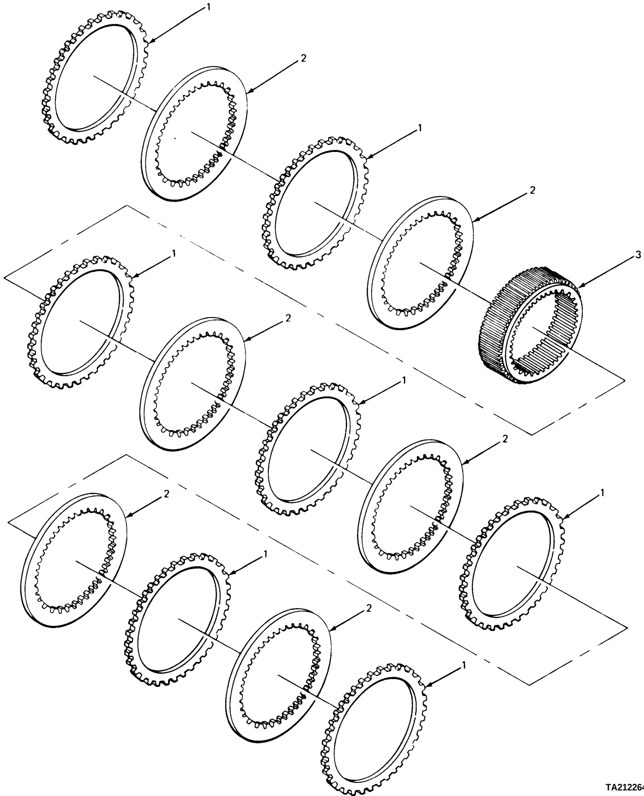
FIGURE 122. RING GEAR AND RELATED PARTS.
