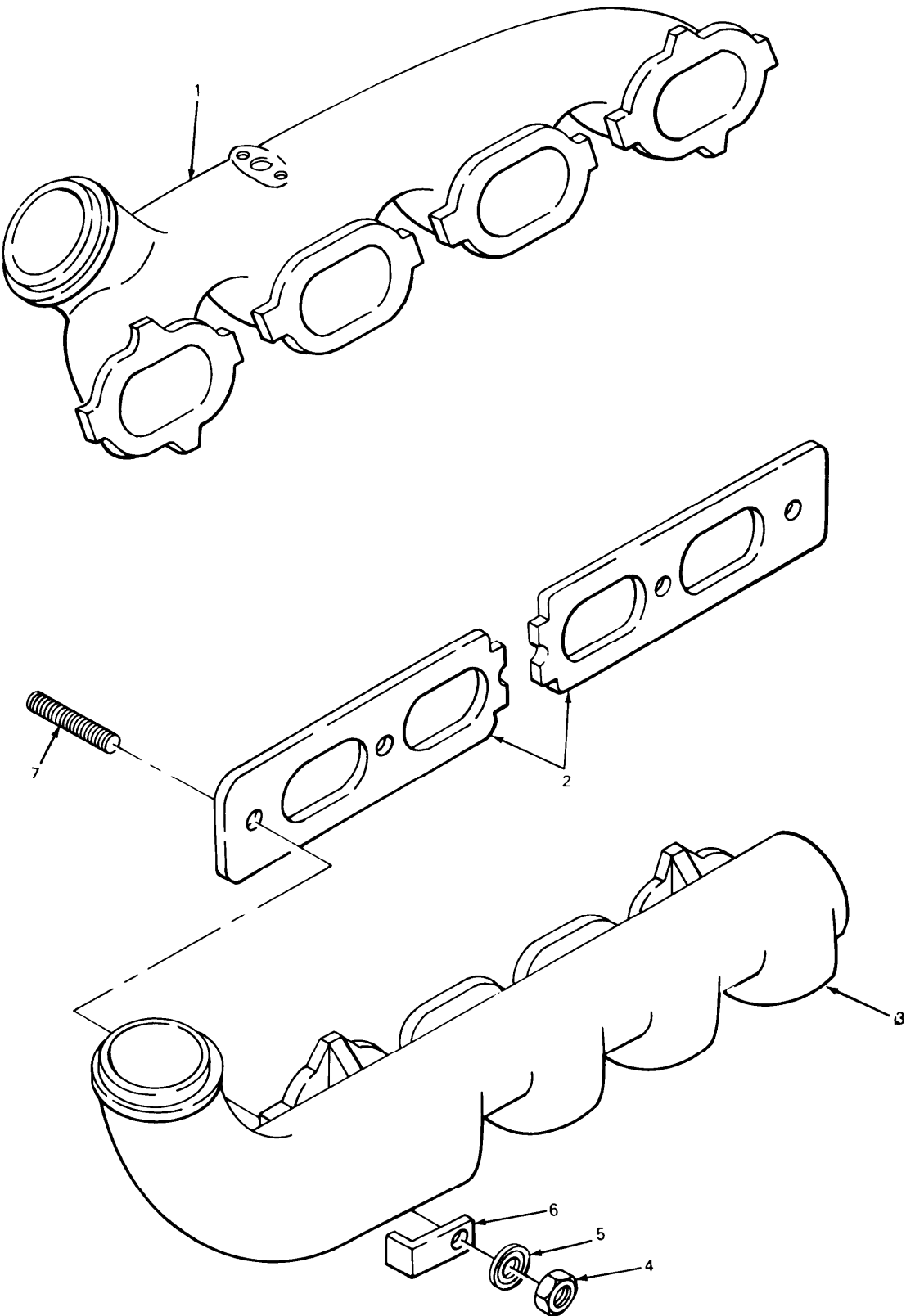
FIGURE 28. EXHAUST MANIFOLDS.
