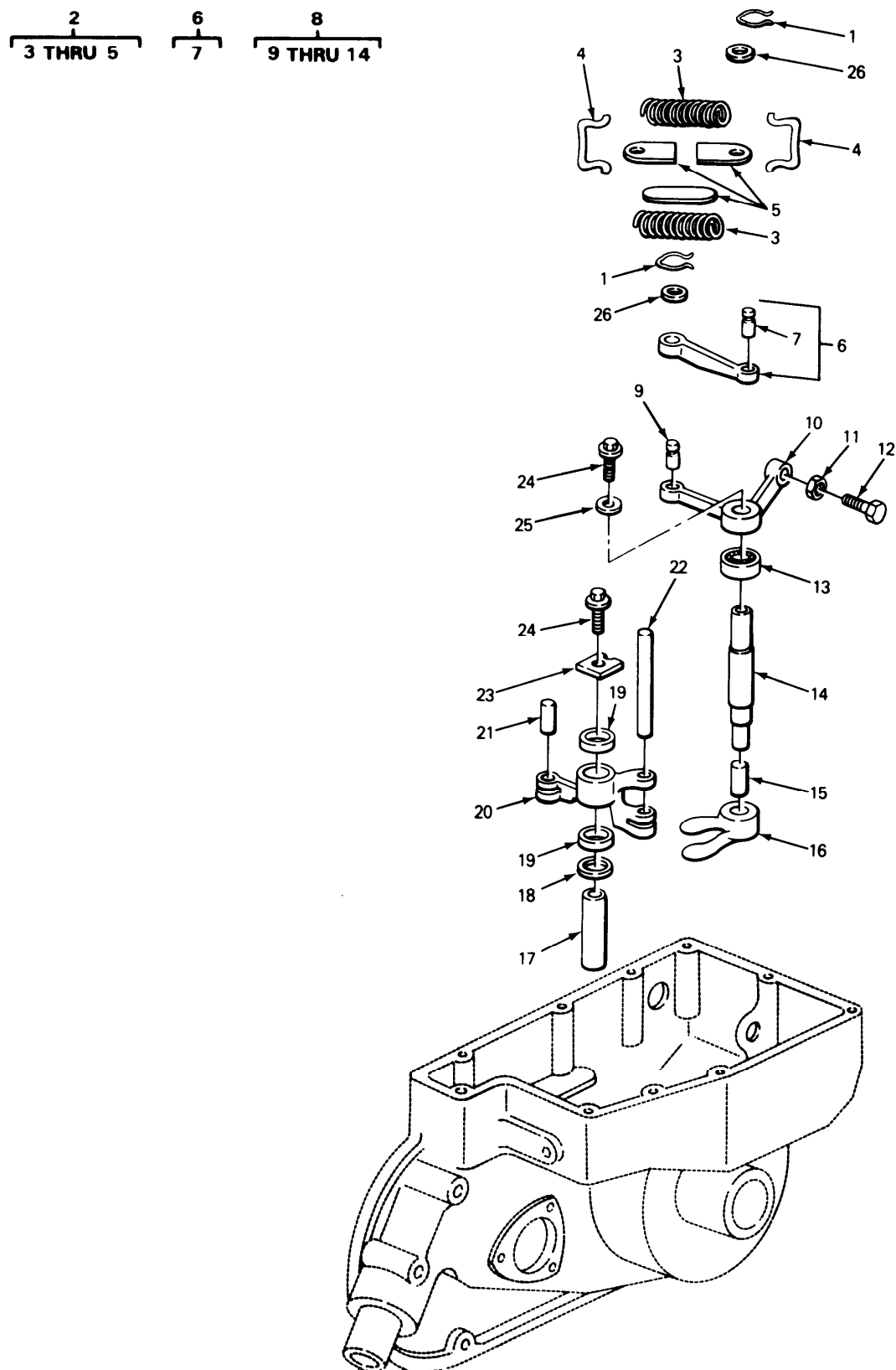
FIGURE 48. GOVERNOR OPERATING SHAFT EXPLODED VIEW.
