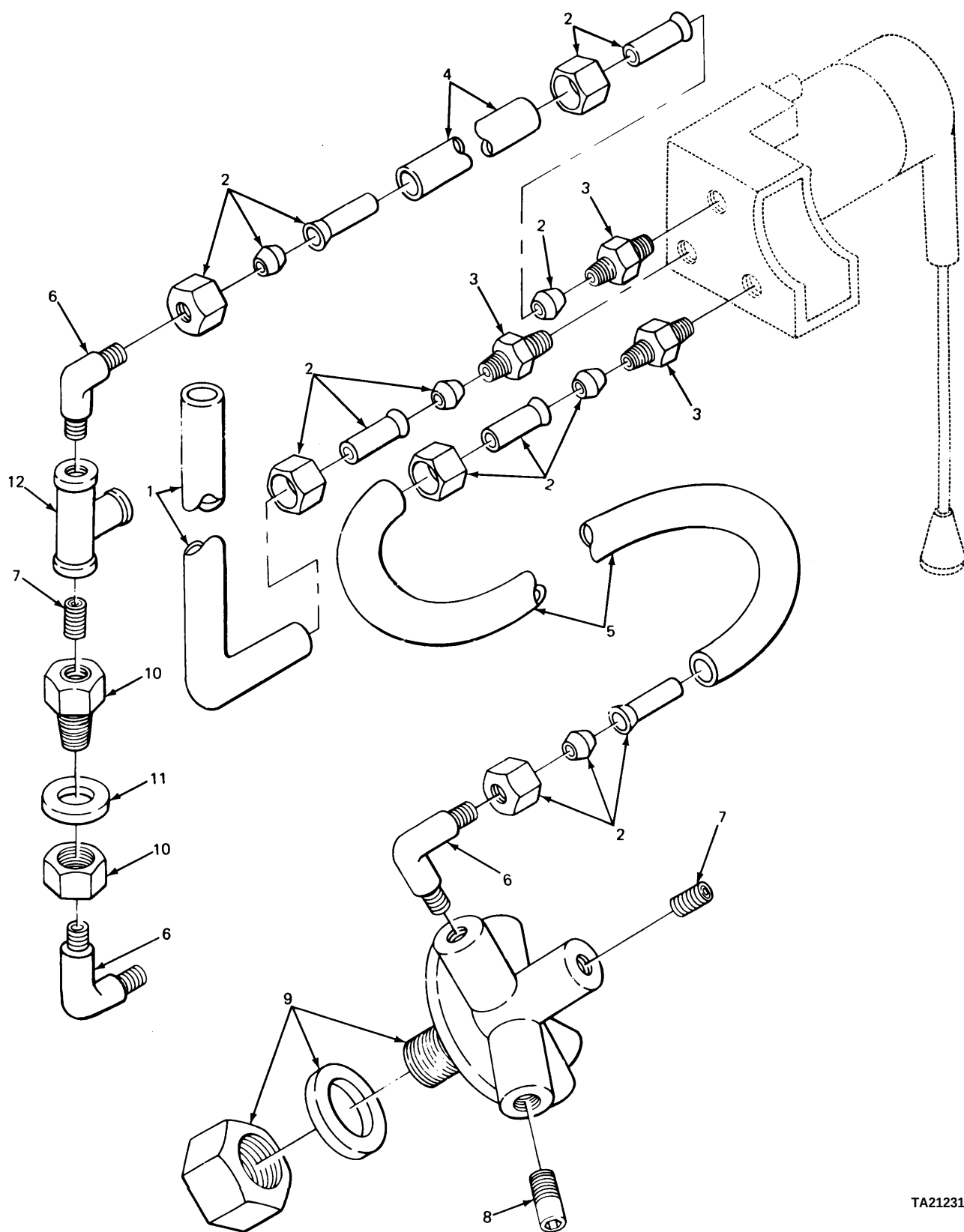
FIGURE 183. BULKHEAD FITTING AND RELATED PARTS.
