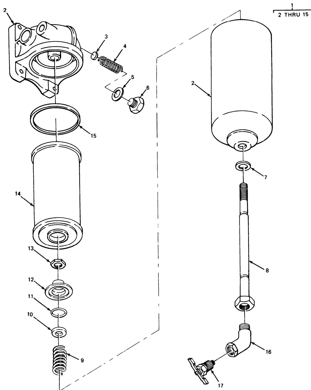
FIGURE 135. EXTERNAL TRANSMISSION OIL FILTER AND RELATED PARTS.
