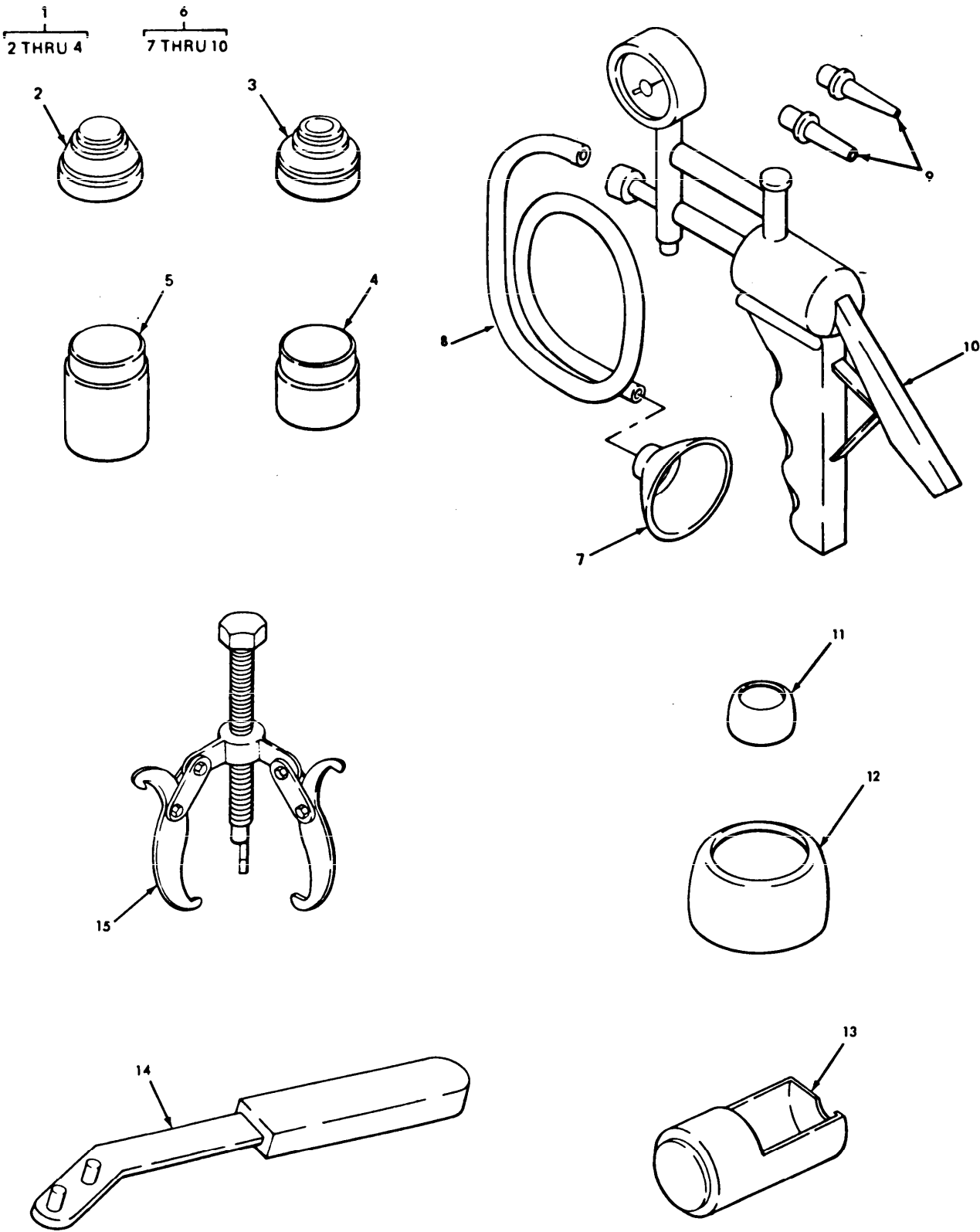
FIGURE 309. GENERAL SUPPORT SPECIAL TOOLS.
