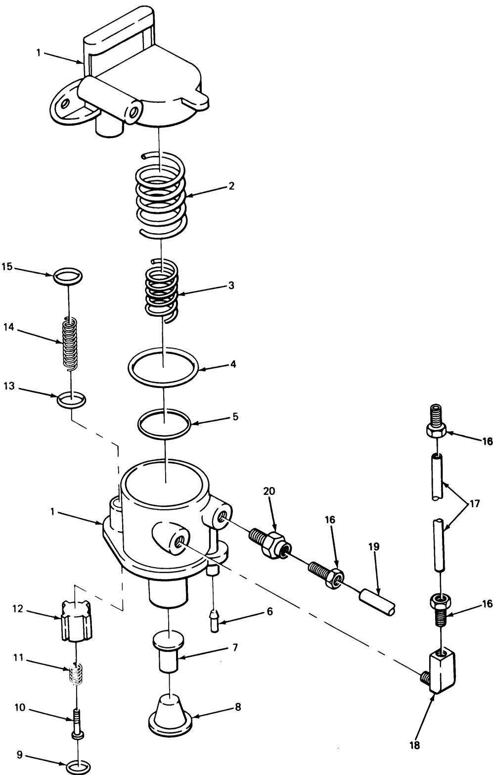
FIGURE 189. SPRING BRAKE VALVE AND RELATED PARTS.
