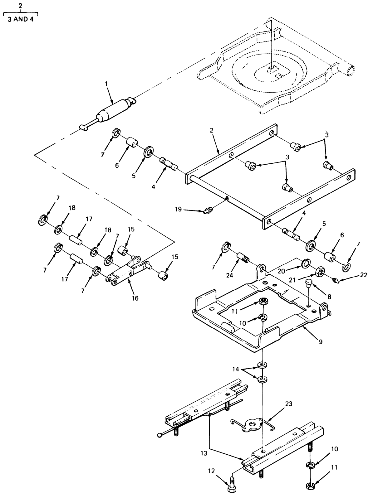
FIGURE 267. BASE ASSEMBLY AND RELATED PARTS.
