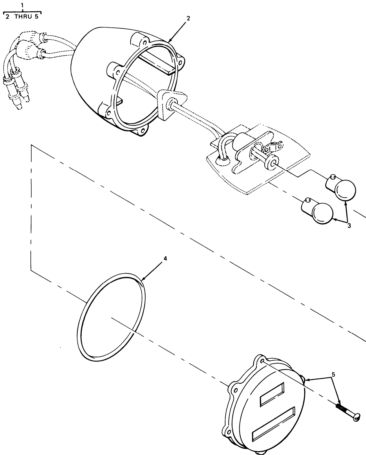
FIGURE 91. BLACKOUT TAILLIGHT.
