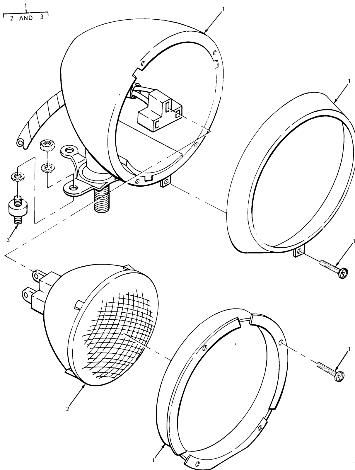
FIGURE 85. HEADLIGHT ASSEMBLY.
