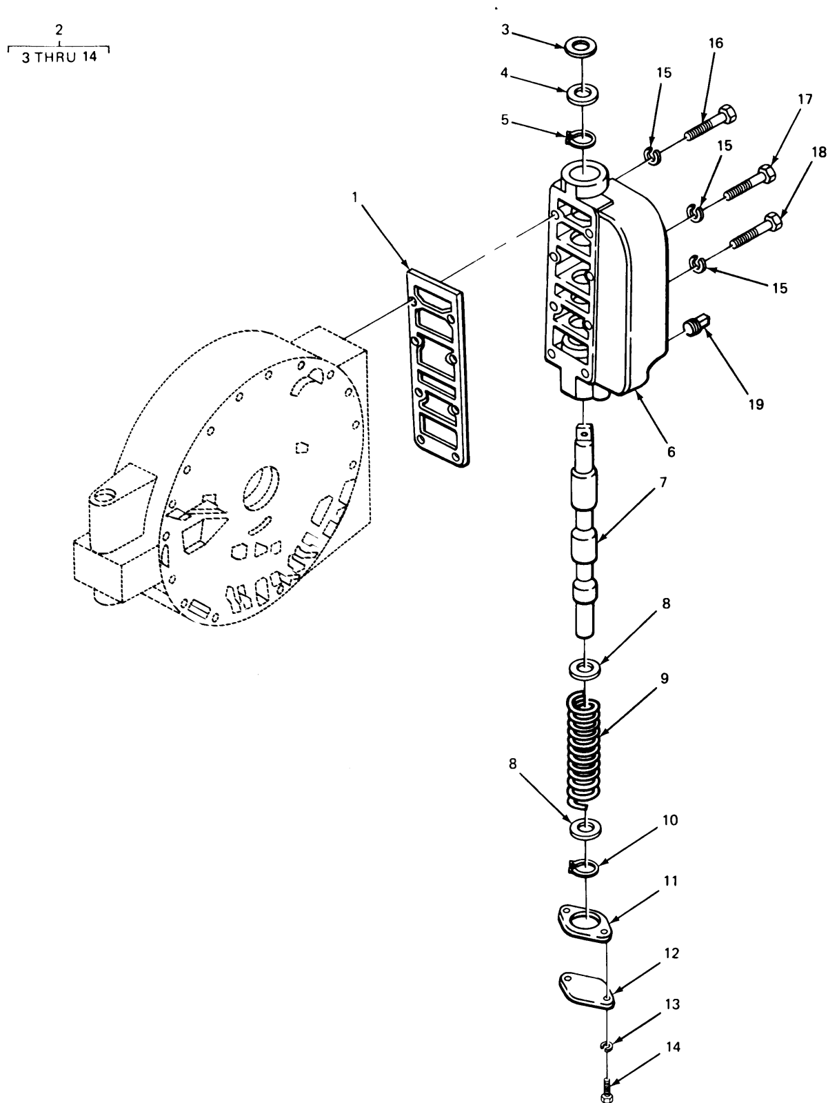
FIGURE 126. RETARDER CONTROL VALVE AND RELATED PARTS.
