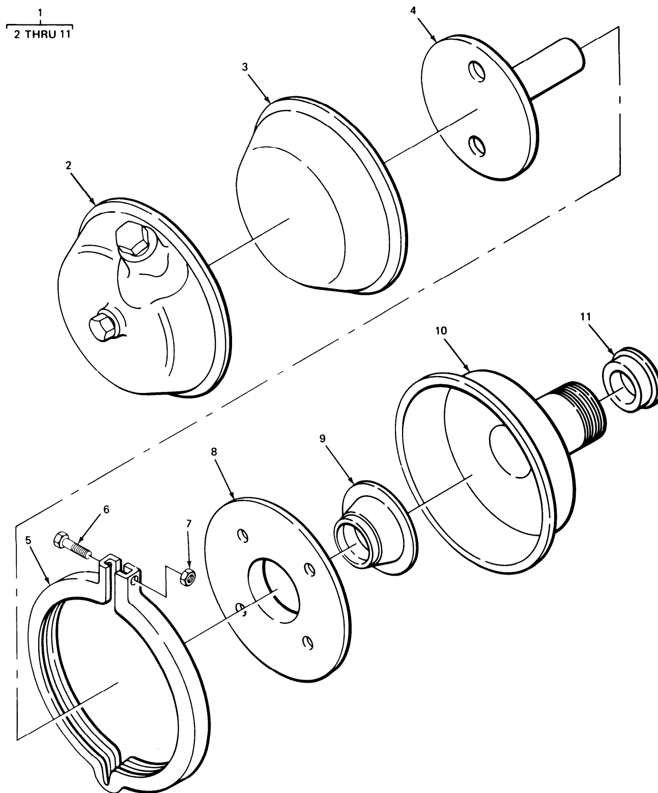
FIGURE 174. PUSHER AXLE AIR BRAKE CHAMBER.
