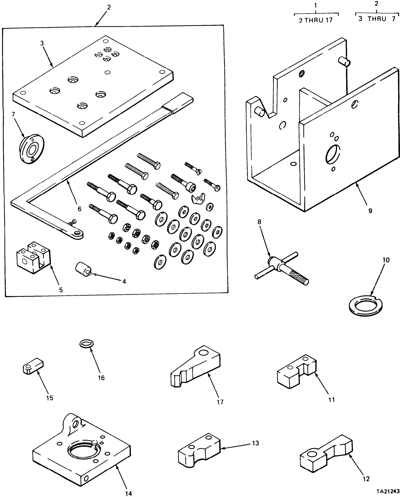
FIGURE 306. DIRECT SUPPORT SPECIAL TOOLS.
