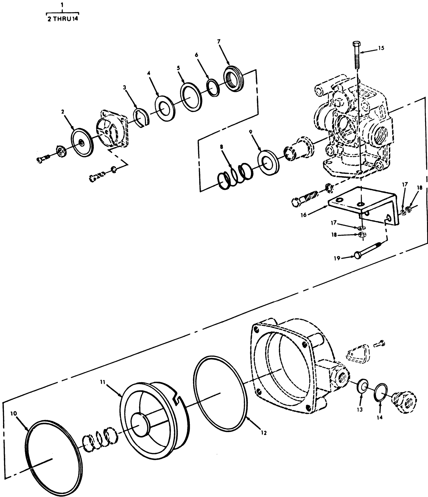
FIGURE 188. RELAY VALVE.
