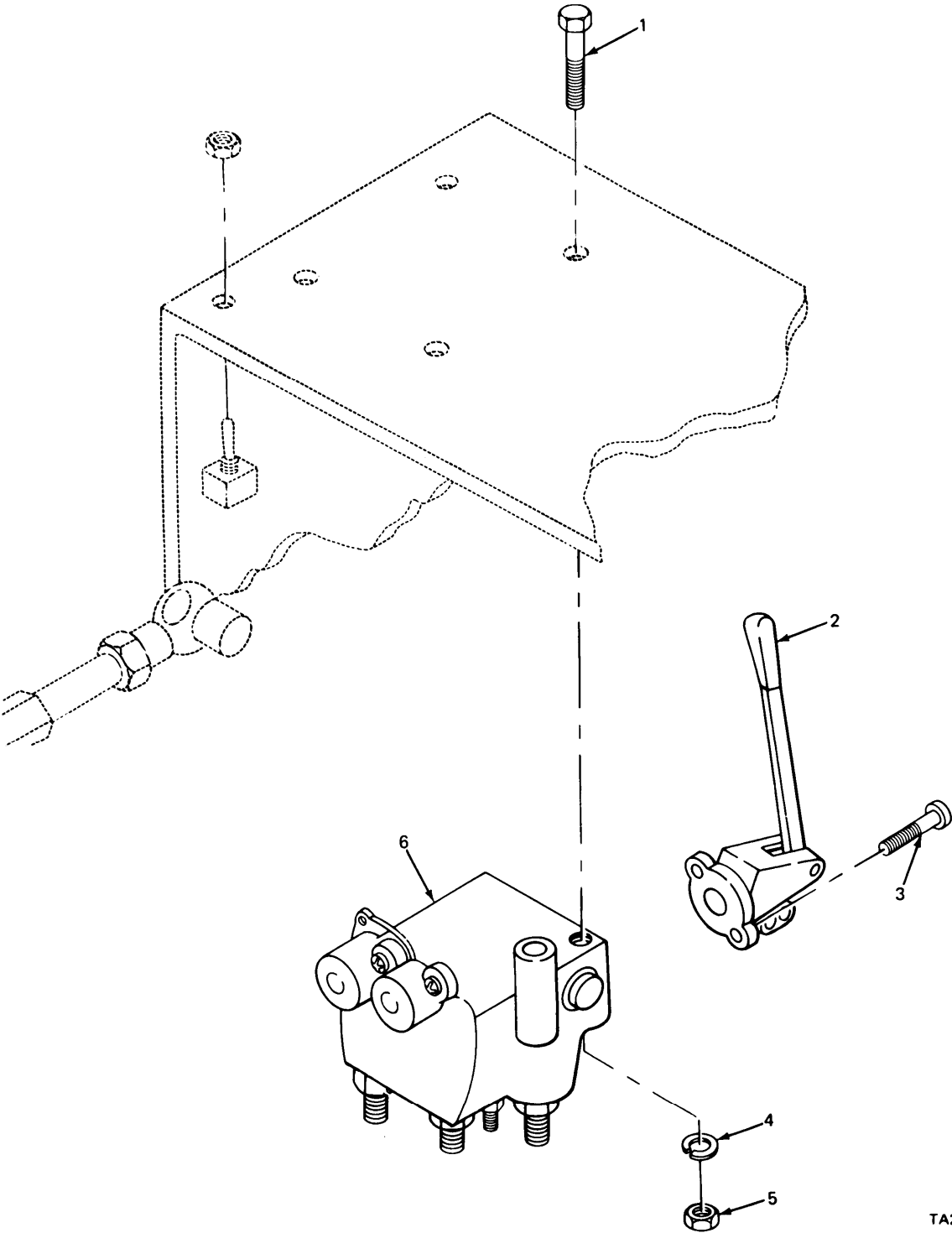
FIGURE 278. WINCH CONTROL.
