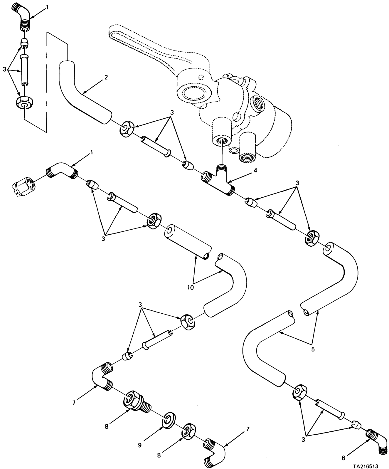
FIGURE 185. TRAILER BRAKE CONTROL LINES AND FITTINGS.
