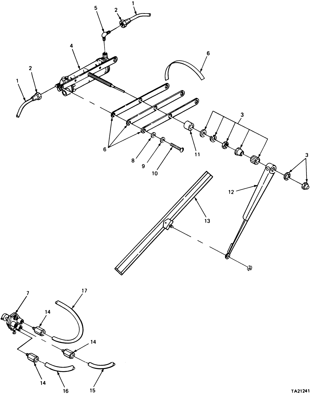
FIGURE 290. WIPER ASSEMBLY.
