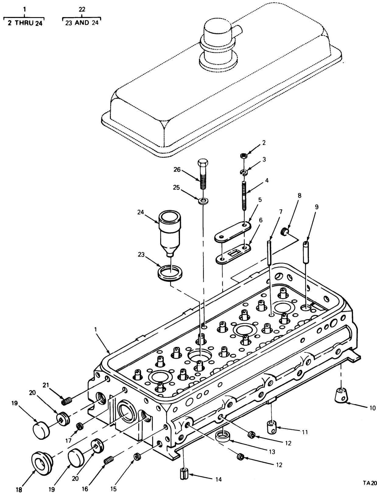
FIGURE 7. CYLINDER HEAD AND RELATED PARTS.
