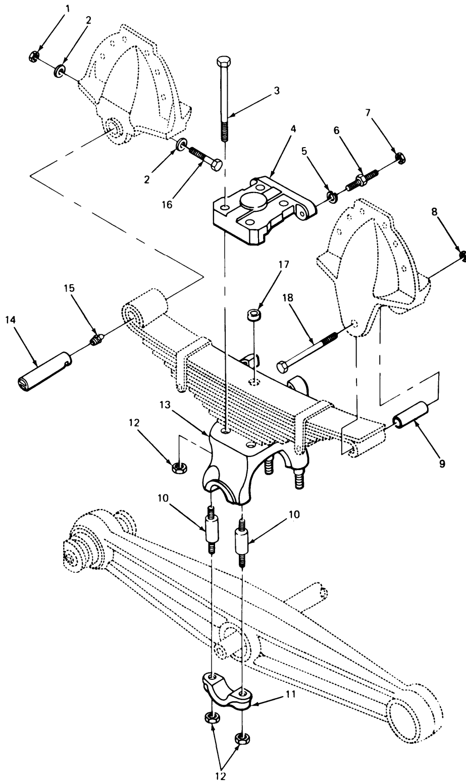
FIGURE 247. TOP SADDLE PLATE AND RELATED PARTS.
